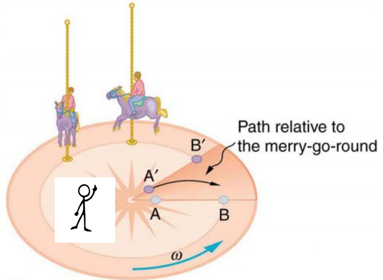
Motion as witnessed by a Non-Inertial Observer
