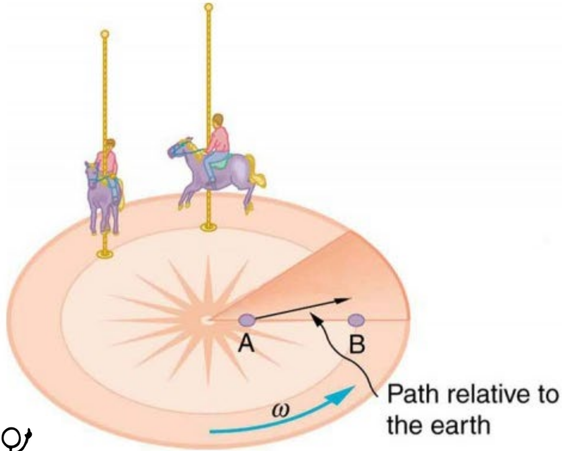
Motion as witnessed by an Inertial Observer
